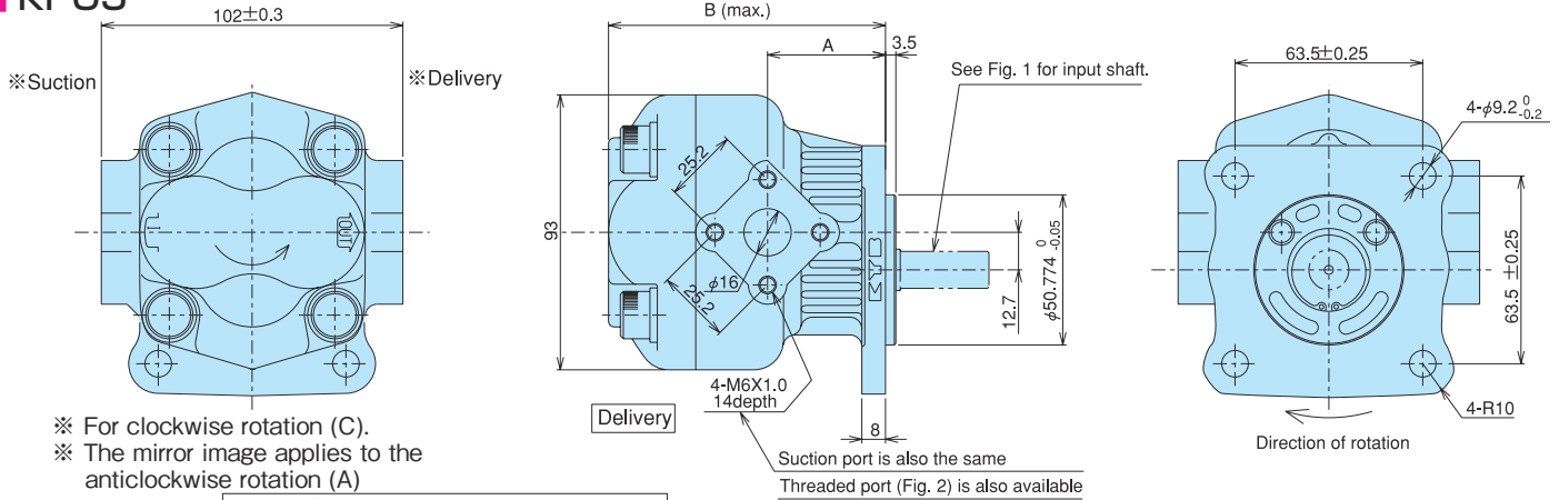
KPO5 displacement, specifications, and dimensions (details)
