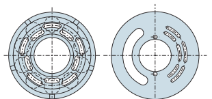
Split flow type cylinder block with each port split into internal and external ports for separate delivery
